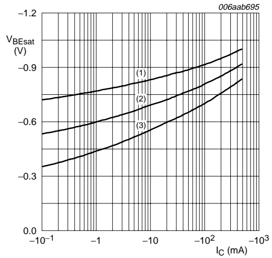
I_C/I_B = 5 (1) T_{amb} = -55^\circ\text{C} (2) T_{amb} = 25^\circ\text{C} (3) T_{amb} = 100^\circ\text{C}
