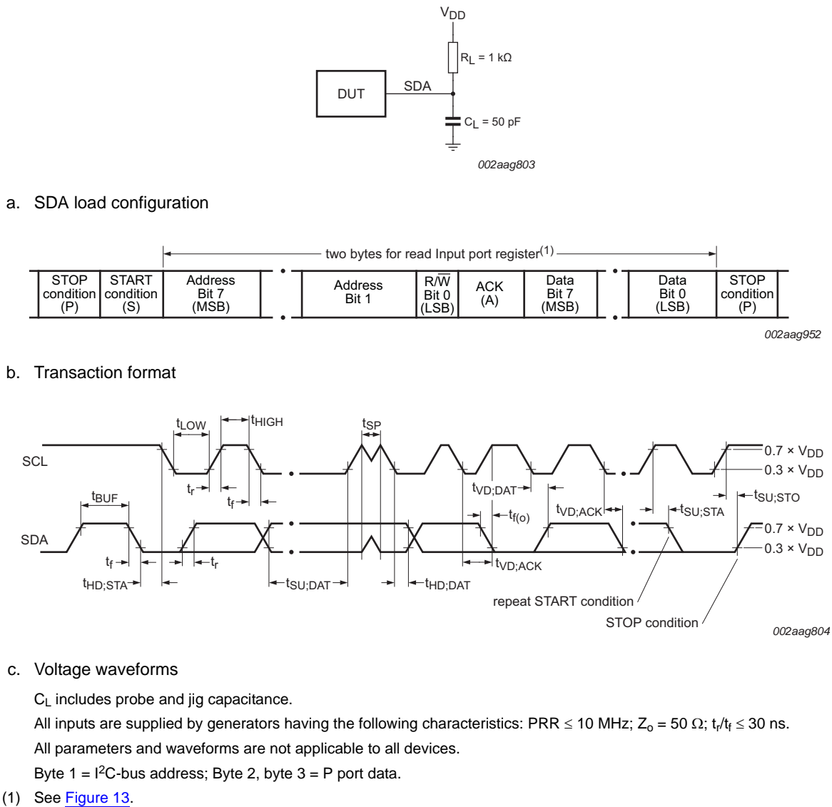
Fig 25. I 2 C-bus interface load circuit and voltage waveforms
