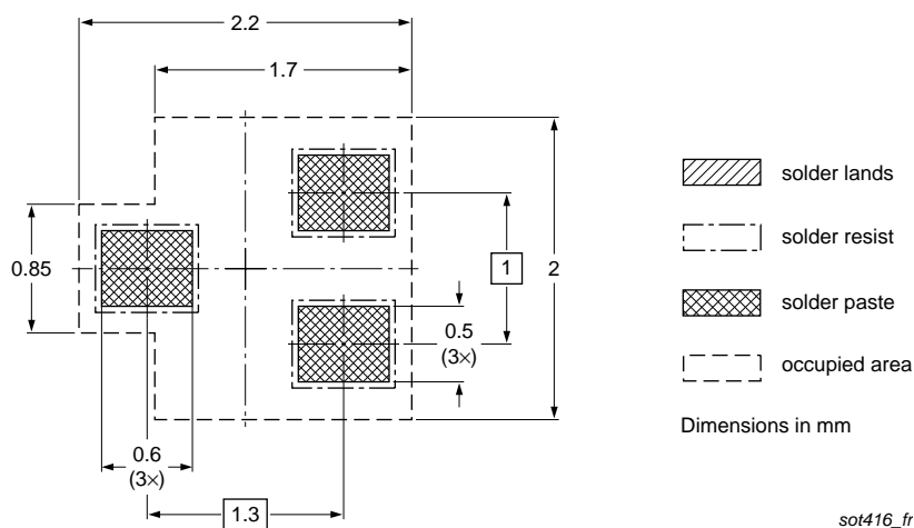
Fig 16. Reflow soldering footprint PDTA114EE (SOT416/SC-75)
