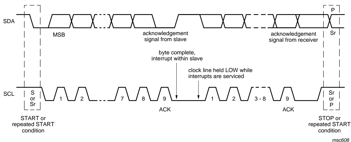
Fig 14. Data transfer on the I 2 C-bus
