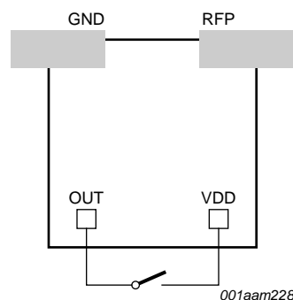
Fig 6. Schematic of connecting VDD and OUT pad with a predetermined breaking point to turn a standard RFID label into a wireless safety seal
