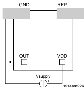
Fig 7. Schematic of external power supply
