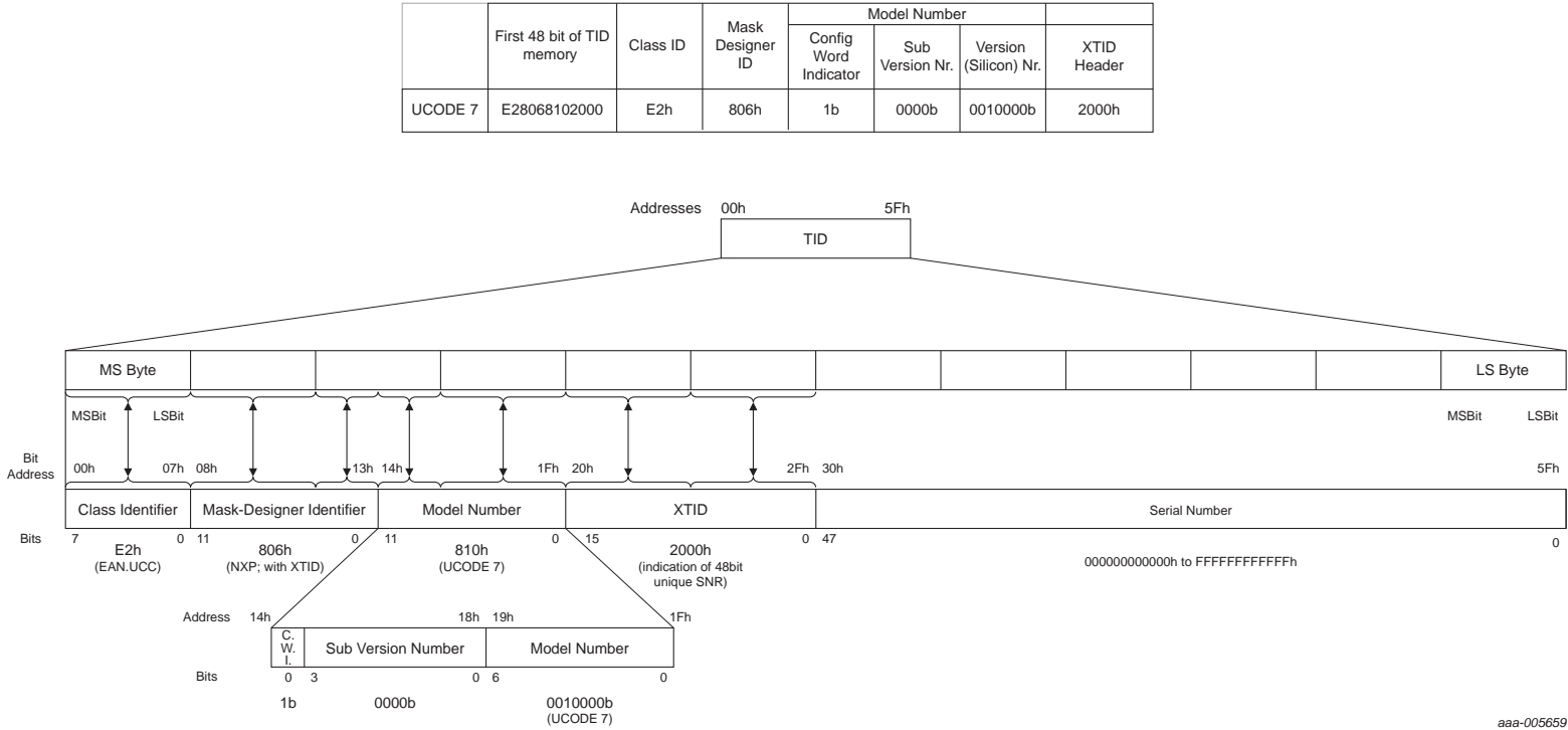
Fig 4. UCODE 7 TID memory structure
