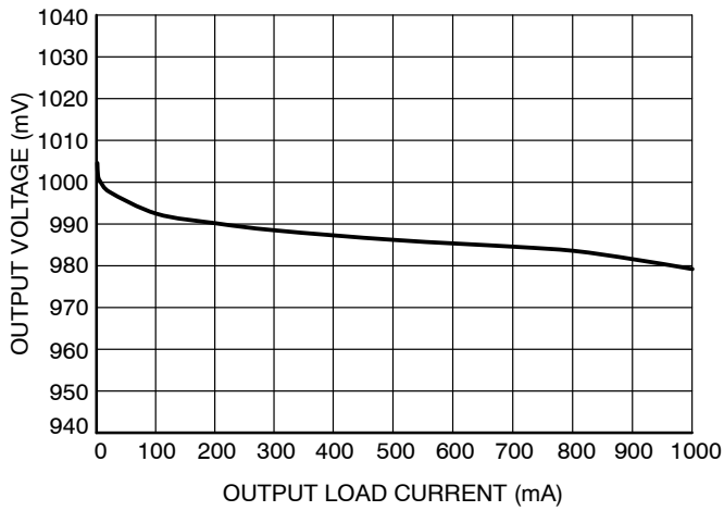
Figure 26. Load Regulation
