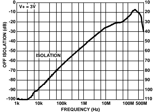
FIGURE 17. OFF-ISOLATION
