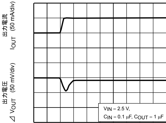
TCR5SB15U ( I_{OUT} = 50 \text{ m to } 100 \text{ mA} )
