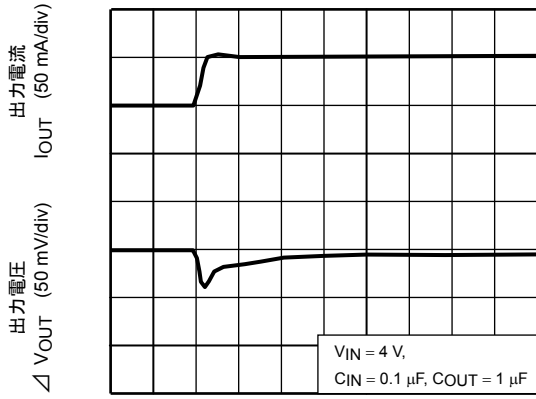
TCR5SB30U ( I_{OUT} = 50 \text{ m to } 100 \text{ mA} )
