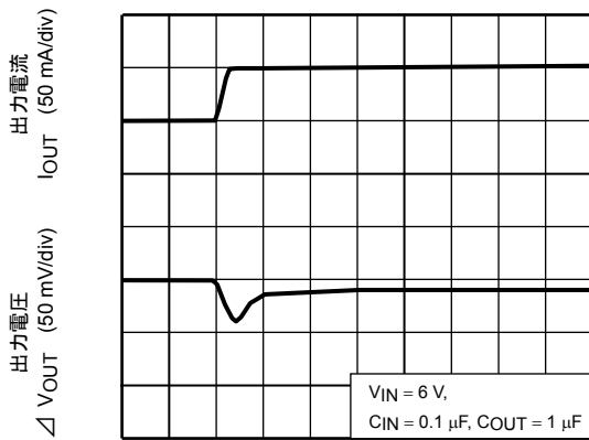
TCR5SB50U ( I_{OUT} = 50 \text{ m to } 100 \text{ mA} )
