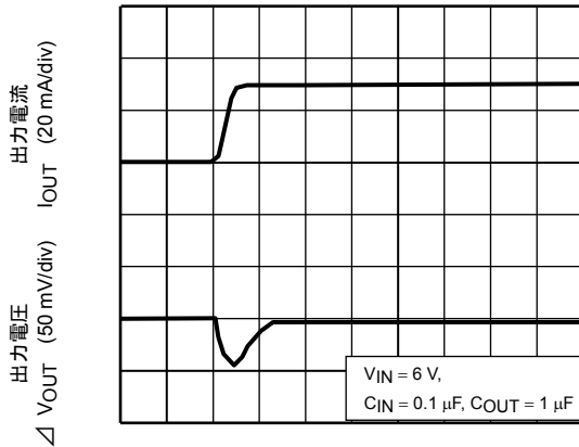
TCR5SB50U ( I_{OUT} = 1 \text{ m to } 30 \text{ mA} )
