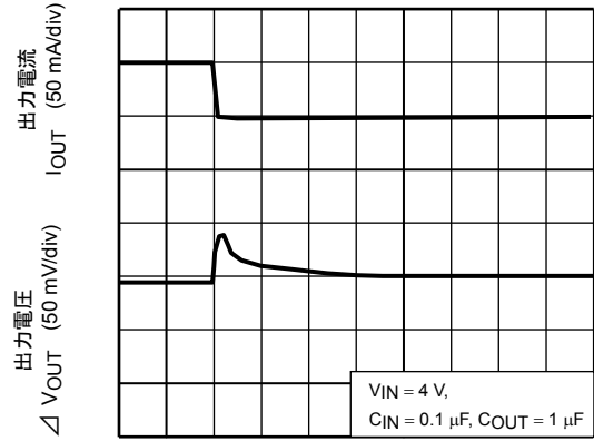
TCR5SB30U ( I_{OUT} = 100 \text{ m to } 50 \text{ mA} )
