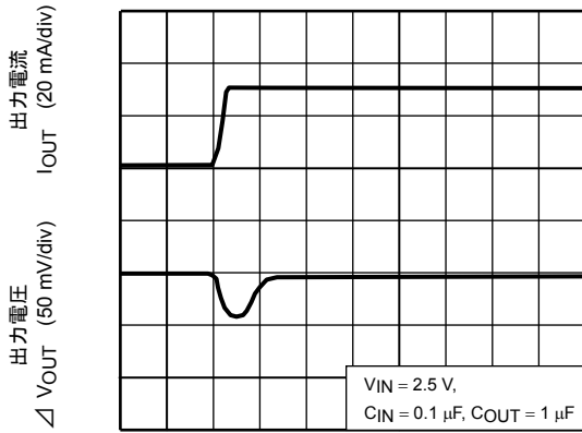
TCR5SB15U ( I_{OUT} = 1 \text{ m to } 30 \text{ mA} )
