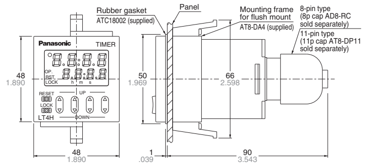
Pin type
