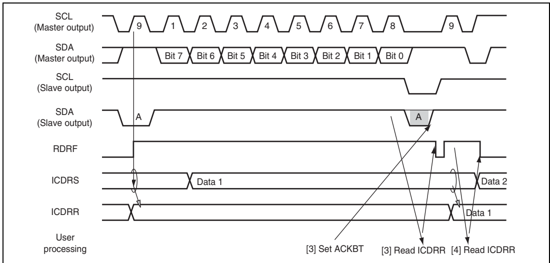
Figure 22.12 Slave Receive Mode Operation Timing (2)
