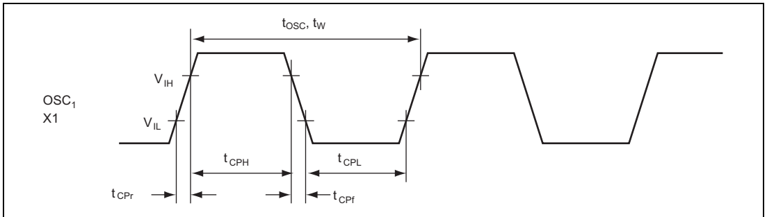
Figure 26.14 Clock Input Timing
