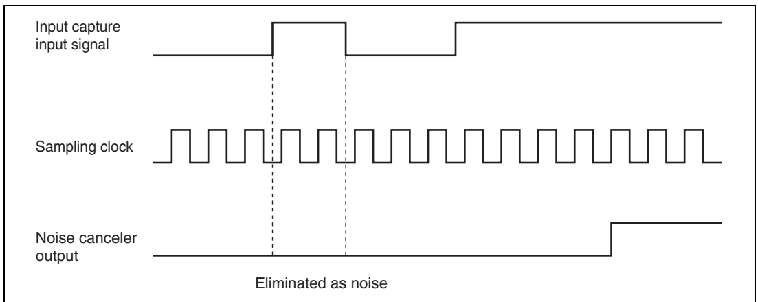
Figure 13.3 Noise Canceller Timing (Example)
