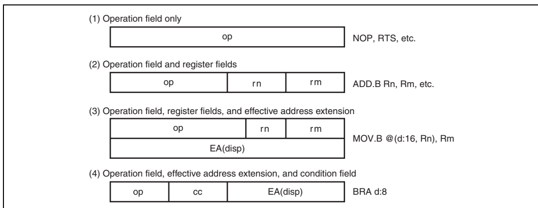
Figure 2.7 Instruction Formats
