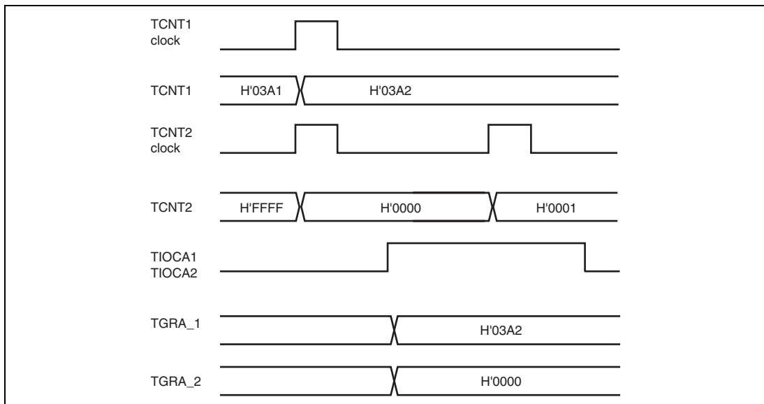
Figure 14.16 Example of Operation with Cascaded Connection
