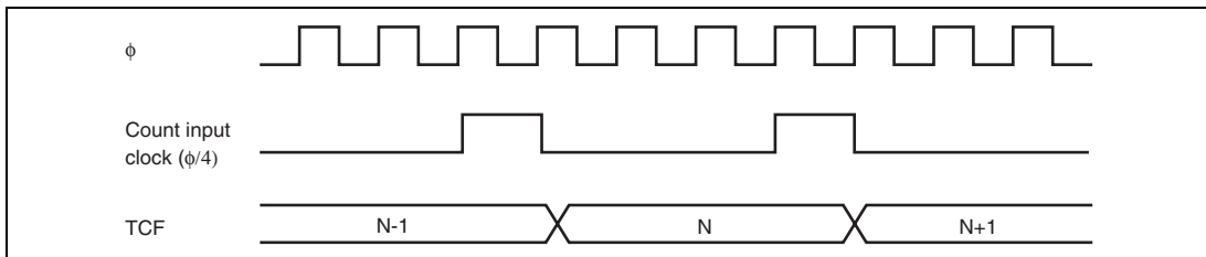
Figure 12.2 Count Timing for Internal Clock Operation
