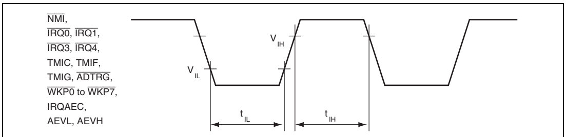
Figure 26.16 Input Timing
