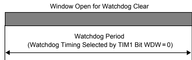
Figure 29. Timeout Watchdog
