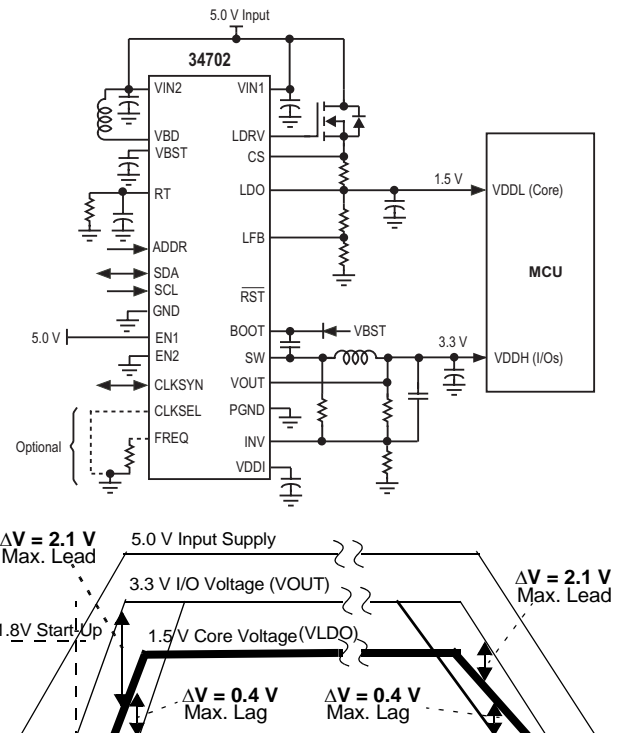
Figure 19. Inverted Power-up/Down Sequence in +5.0V Supply System
