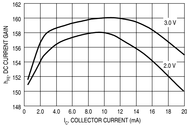
Figure 3. h FE , DC Current Gain versus Collector Current
