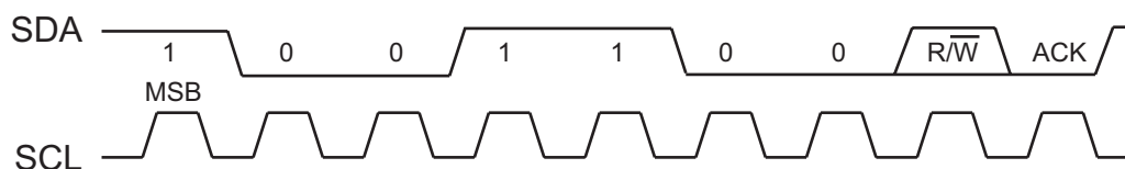
Figure 9. Slave Address
