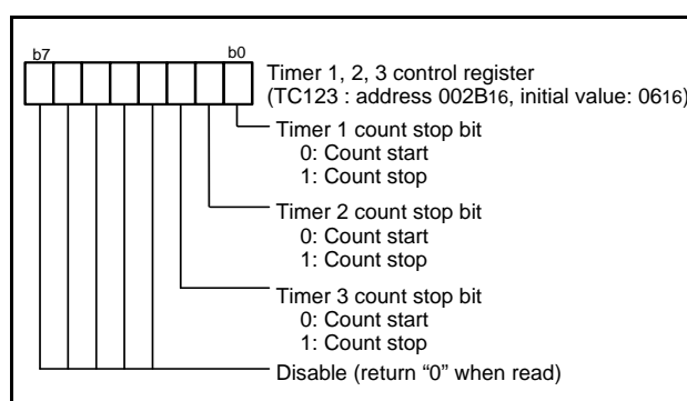
Fig. 23 Timer 1, 2, 3 control register
