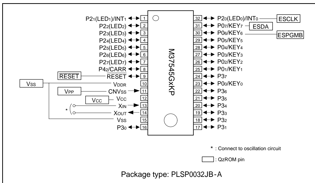
Fig. 45 Pin connection diagram (M37545GxKP)
