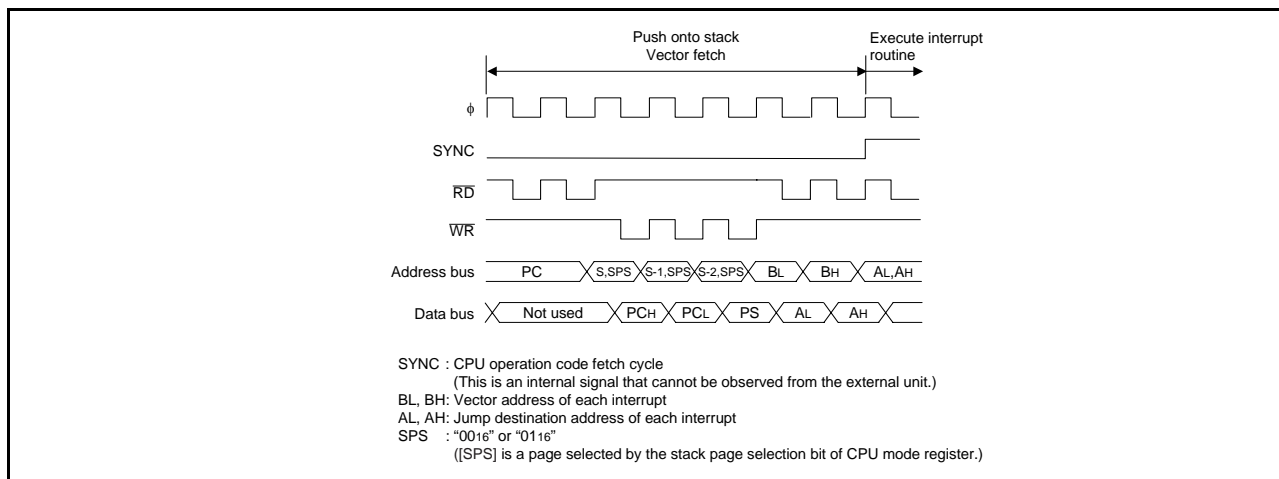
Fig. 19 Interrupt sequence
