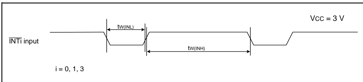
Figure 5.11 External Interrupt \overline{\text{INT}}_i Input Timing Diagram when Vcc = 3 V
