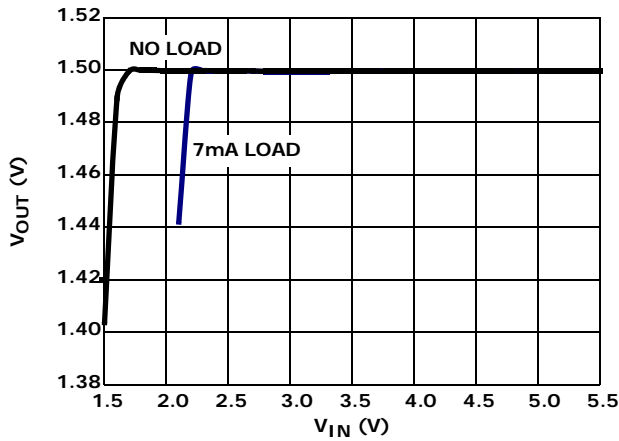
FIGURE 11. DROPOUT
