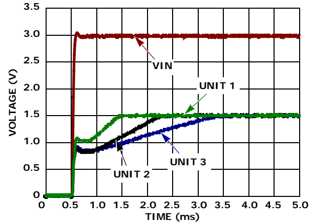
FIGURE 12. TURN-ON TIME
