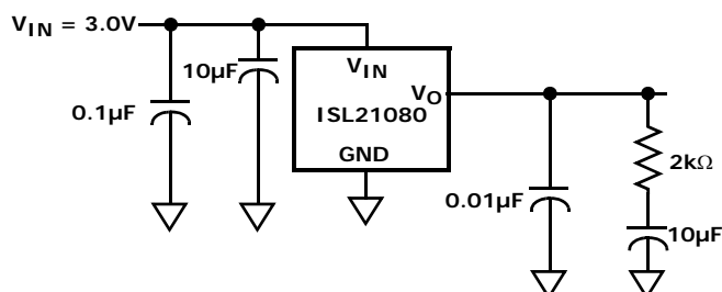
FIGURE 20. NOISE REDUCTION NETWORK
