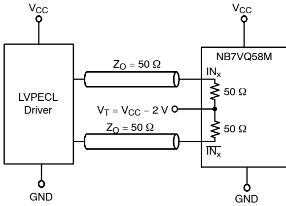
Figure 13. LVPECL Interface
