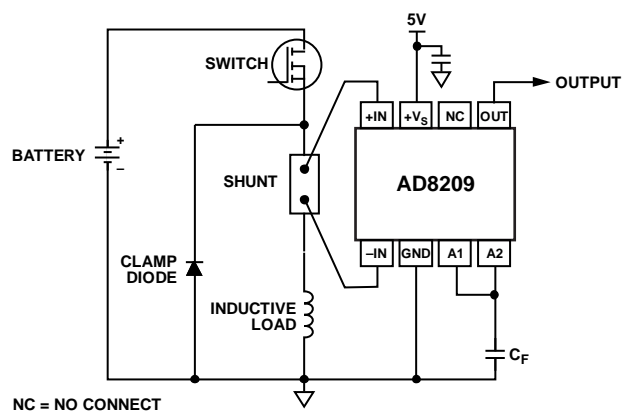
Figure 25. High-Side Switch
