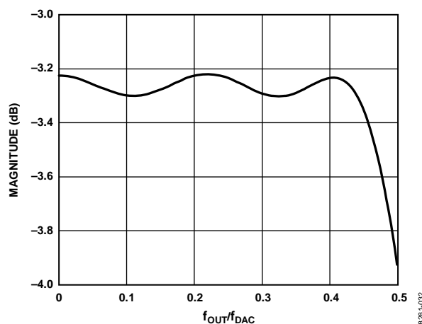
Figure 60. Sample Composite Responses of the \text{Sinc}^{-1} Filter with \text{Sin}(x)/x Roll-Off
