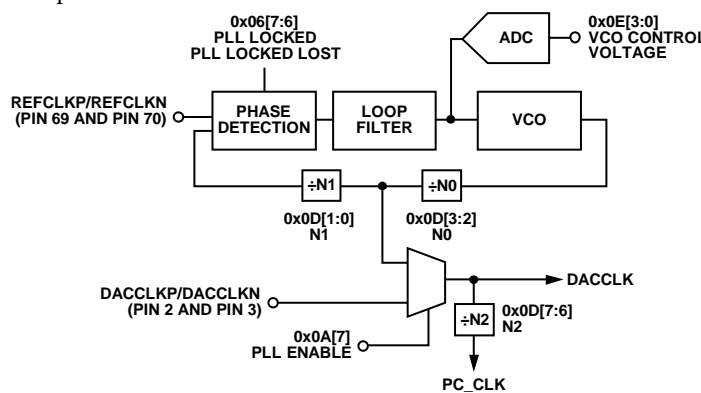
Figure 62. PLL Clock Multiplication Circuit
