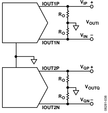
Figure 66. Basic Transmit DAC Output Circuit
