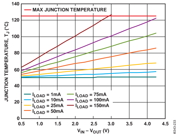
Figure 38. TSOT, 0 mm 2 of PCB Copper, T A = 50°C
