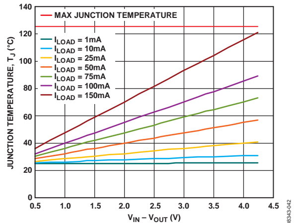
Figure 40. WLCSF, 500 mm 2 of PCB Copper, T A = 25°C
