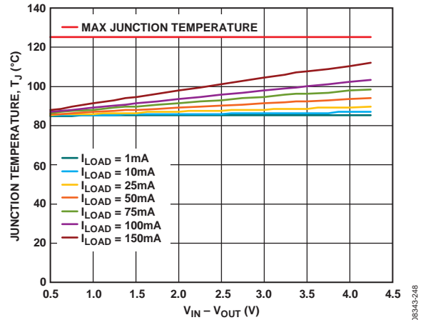
Figure 39. TSOT, 100 mm 2 of PCB Copper, Board Temperature = 85°C
