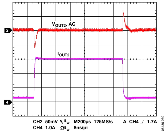
Figure 39. Load Transient Response in Pulse Skip Mode, Channel 2: 0.3 A to 3 A Load Step, V_{IN} = 3.3 V, V_{OUT} = 1.2 V, f_{SW} = 1.2 MHz (See Table 12 for the Circuit Details)
