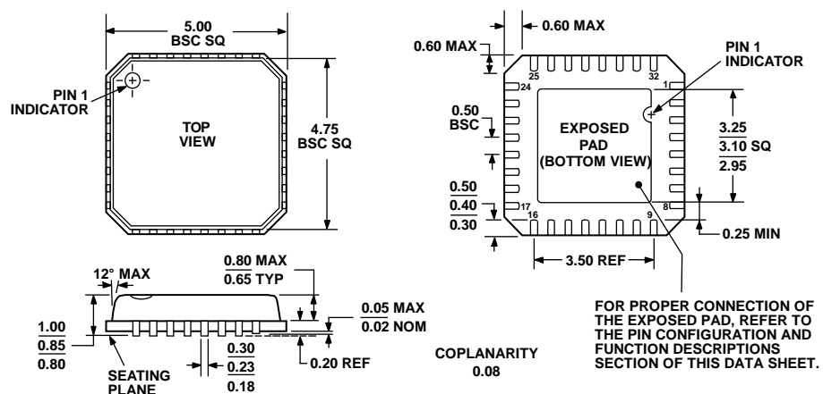
Figure 77. 32-Lead Lead Frame Chip Scale Package [LFCSP_VQ] 5 mm x 5 mm Body, Very Thin Quad (CP-32-2) Dimensions shown in millimeters
