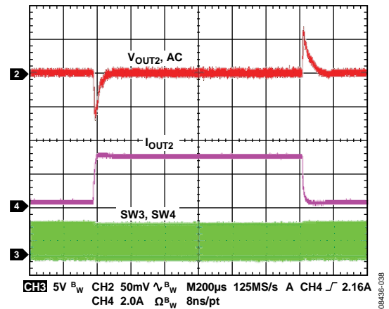
Figure 38. Load Transient Response in Pulse Skip Mode, Channel 2: 0.3 A to 3 A Load Step, V_{IN} = 5 V, V_{OUT} = 1.2 V, f_{SW} = 600 kHz (See Table 12 for the Circuit Details)
