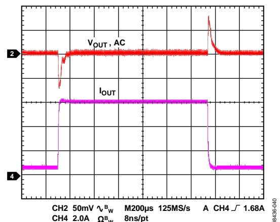
Figure 40. Load Transient Response in Forced PWM Mode, Combined Output: 0.6 A to 6 A Load Step, V_{IN} = 5 V, V_{OUT} = 1.2 V, f_{SW} = 600 kHz (See Table 12 for the Circuit Details)
