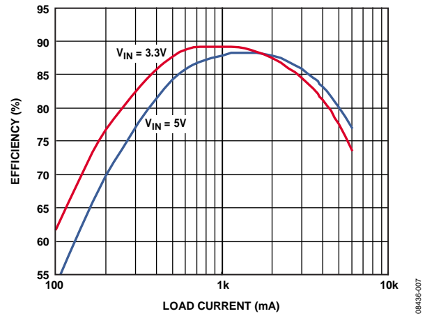
Figure 7. Efficiency, Combined Dual-Phase Output, V_{OUT} = 1.2\text{ V} and f_{SW} = 1.2\text{ MHz} ; Inductor TOKO FDV0620-1R0M, 1.0\text{ }\mu\text{H} , 14\text{ m}\Omega
