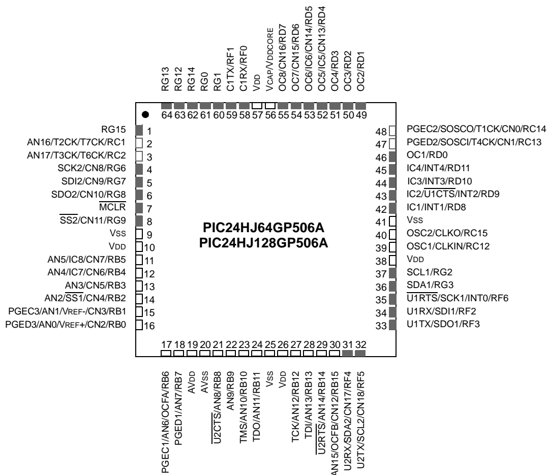
64-Pin QFN (1)
