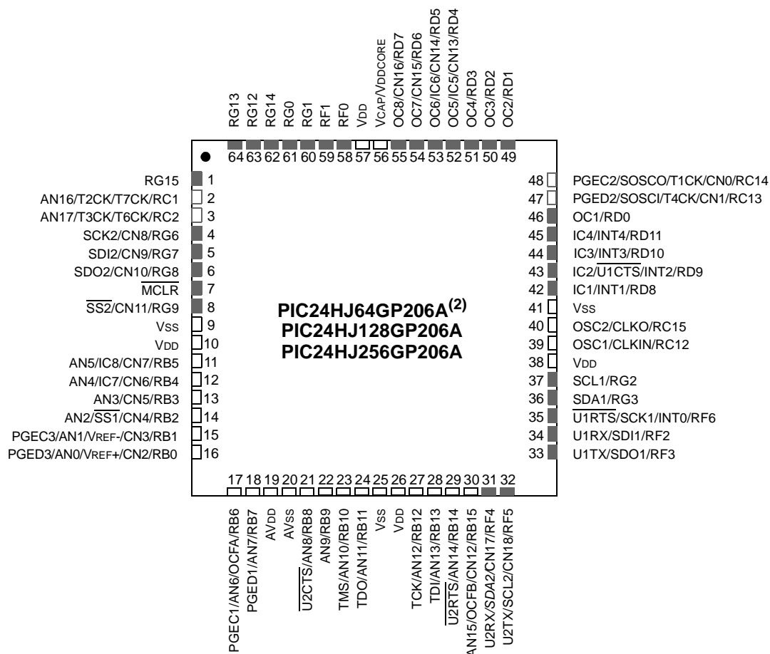
64-Pin QFN (1)
