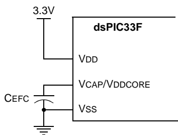
FIGURE 22-1: CONNECTIONS FOR THE ON-CHIP VOLTAGE REGULATOR (1)
