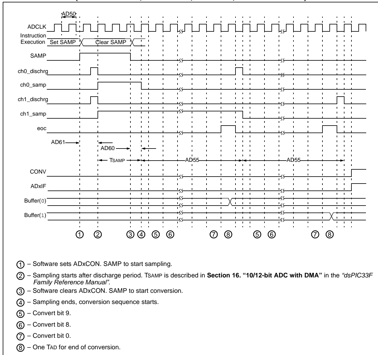
FIGURE 26-24: ADC CONVERSION (10-BIT MODE) TIMING CHARACTERISTICS (CHPS<1:0> = 01, SIMSAM = 0, ASAM = 0, SSR<2:0> = 000)
