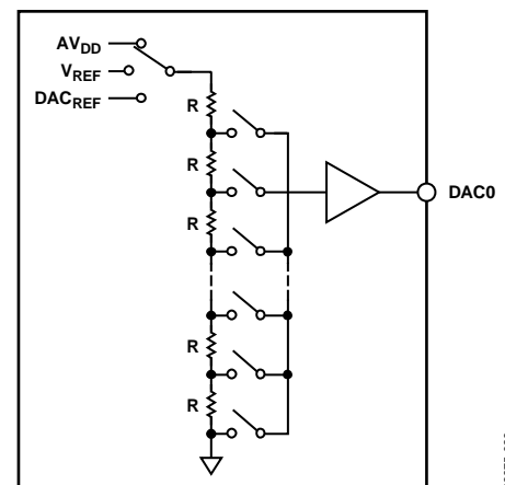
Figure 32. DAC Structure
