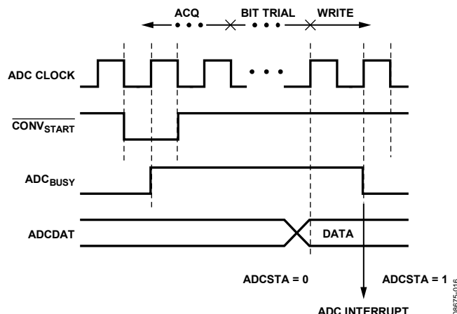
Figure 22. ADC Timing
