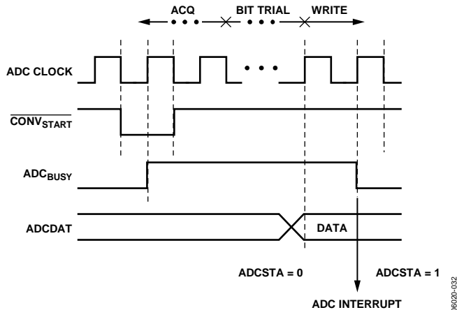
Figure 16. ADC Timing
