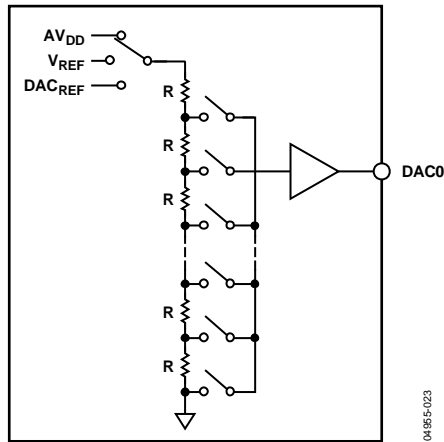
Figure 29. DAC Structure
