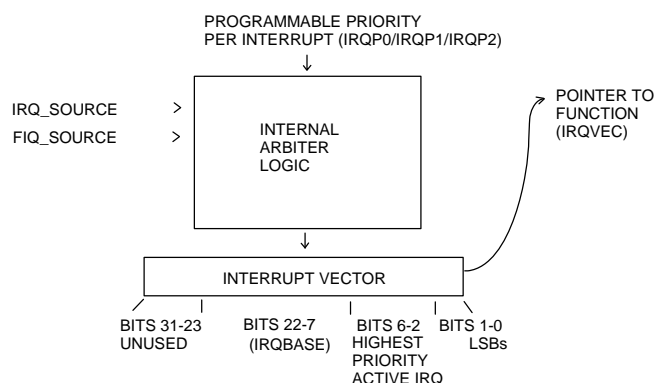
Figure 36. Interrupt Structure
