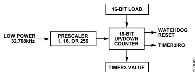
Figure 37. Timer3 Block Diagram
