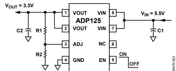
Figure 2. ADP125 with Adjustable Output Voltage
