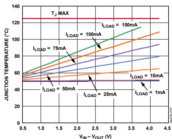
Figure 37. Junction Temperature vs. Power Dissipation, 1000 mm 2 of PCB Copper, T_A = 50^\circ\text{C}
