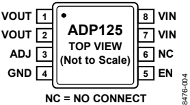
Figure 4. ADP125 Adjustable Output Pin Configuration
