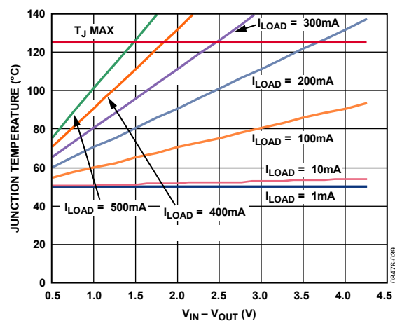
Figure 39. Junction Temperature vs. Power Dissipation, 40 mm 2 of PCB Copper, T_A = 50^\circ\text{C}
