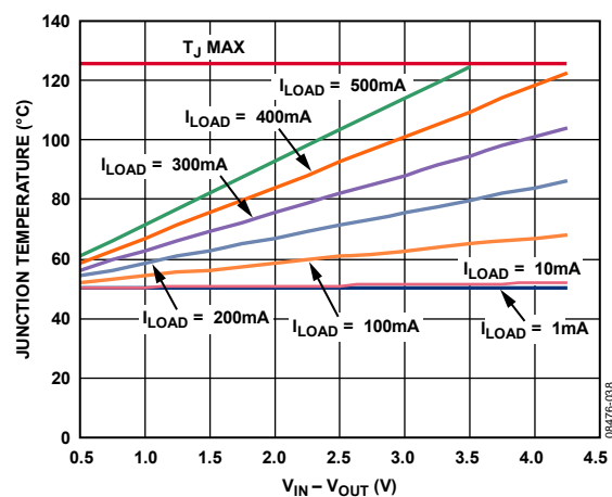
Figure 38. Junction Temperature vs. Power Dissipation, 500 mm 2 of PCB Copper, T_A = 50^\circ\text{C}
