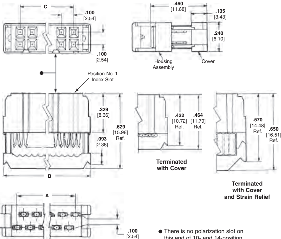
Housing Assembly and Cover
