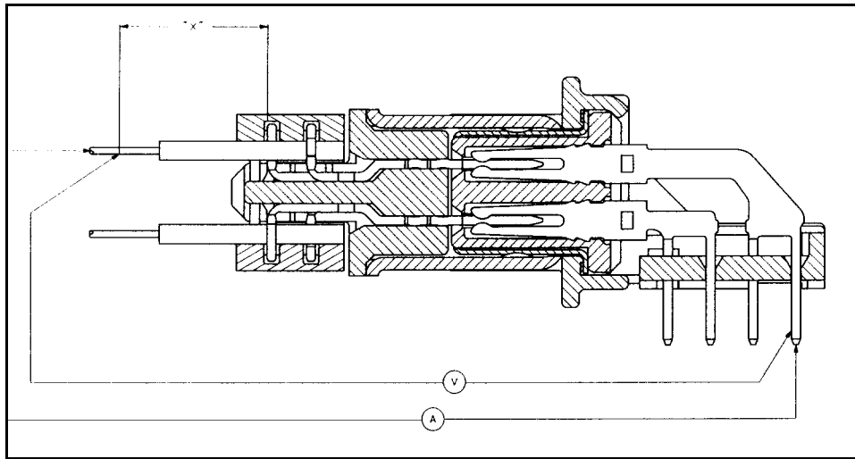
Figure 5 Termination Resistance Measurement Points
