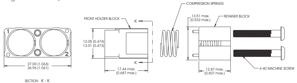
MINI-E BEAM HOLDER KIT Holder Kit, Pin (Spring-Loaded), Mini-Expanded Beam, Key A GPRB 1445162-1
