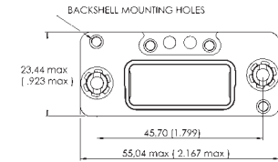
Plug Without Grounding Block GPRB1PB05N
