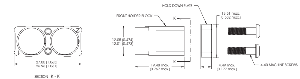
MINI-E BEAM HOLDER KIT Holder Kit, Socket (Fixed), Mini-Expanded Beam, Key A GPRB 1445163-1
