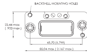
Plug With Grounding Block GPRB1WB05N
