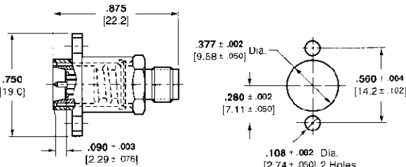
Nickel Plated Part No. 448091-1 Stainless Steel Part No. 448091-2
