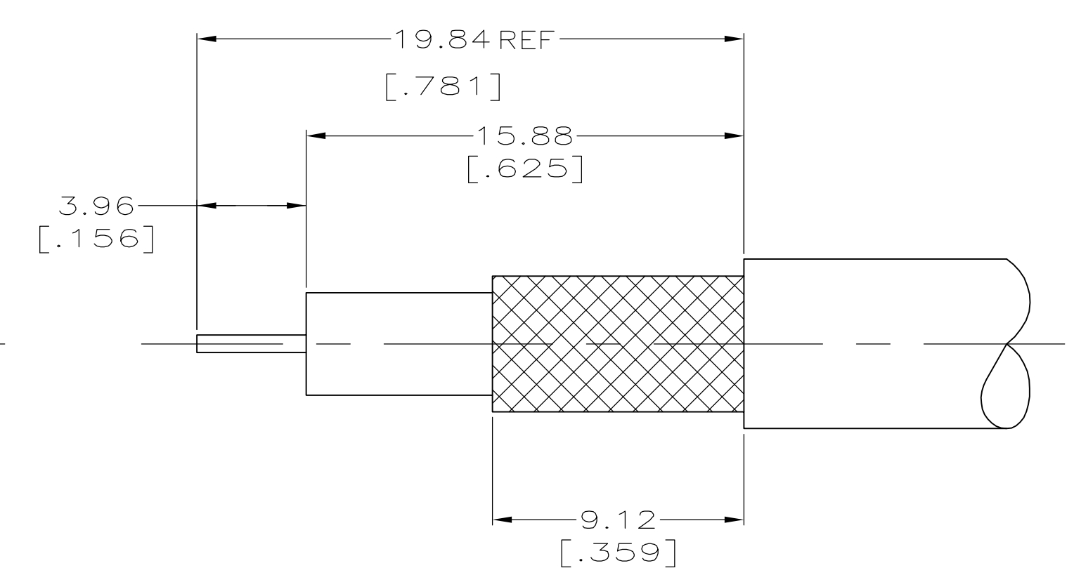
VIEW B
