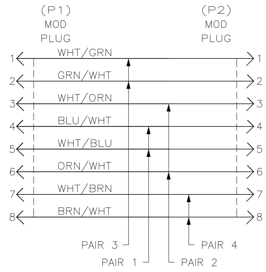
WIRING DIAGRAM 568A 6
