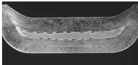
Cross Section of Bar Crimp
