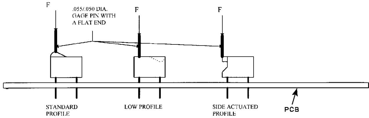
Figure 4 Actuation Force
