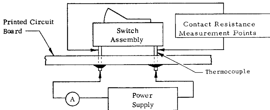
Figure 3 Temperature & Resistance Measurement Points, Typical
