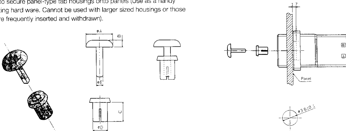
Recommended panel hole dimension
