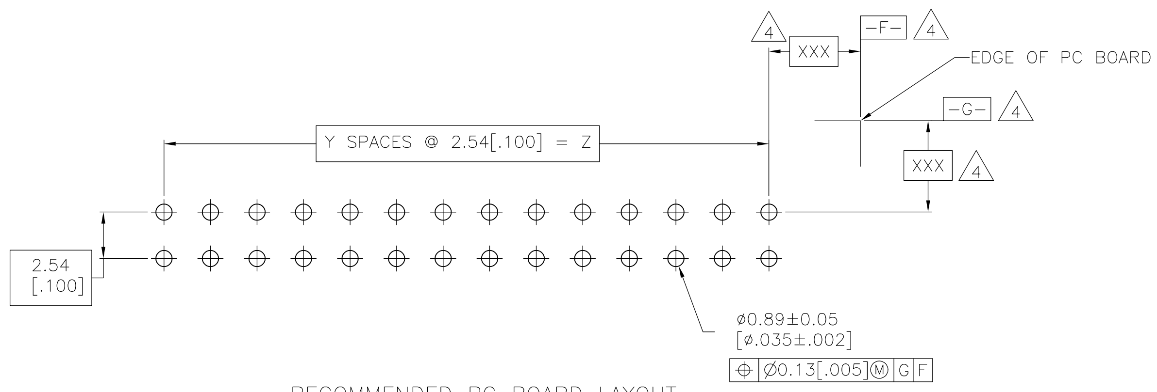
RECOMMENDED PC BOARD LAYOUT 1.57[.062] PC BOARD VIEWED FROM CONNECTOR SIDE
