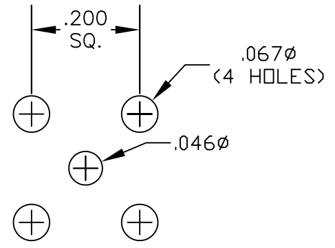
MOUNTING HOLES
