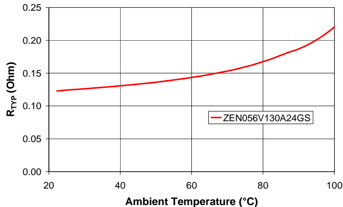
Temperature Effect on R TP
