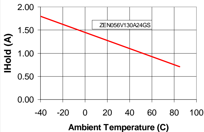
Temperature Effect on I Hold (I FLT = 0)
