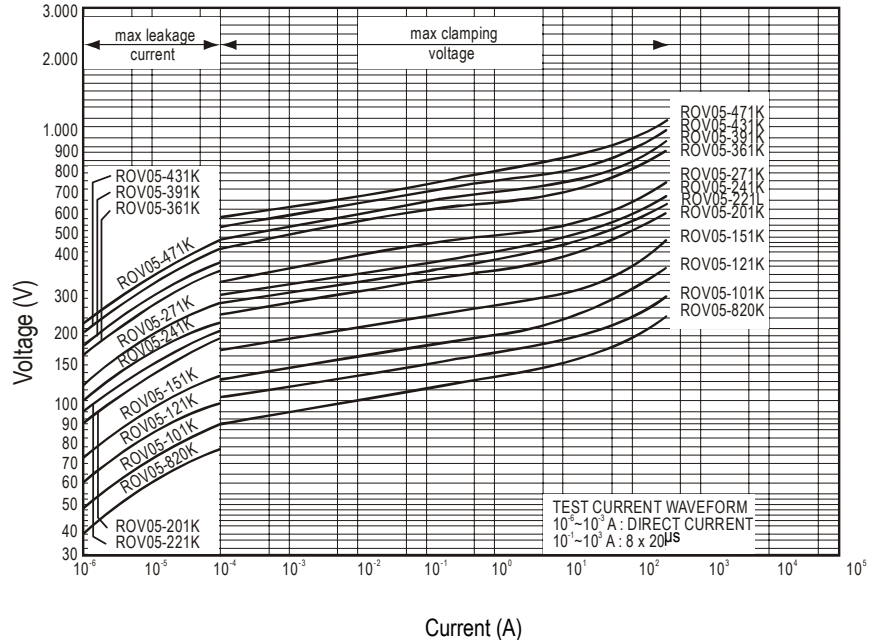
ROV05-820K – ROV05-471K
