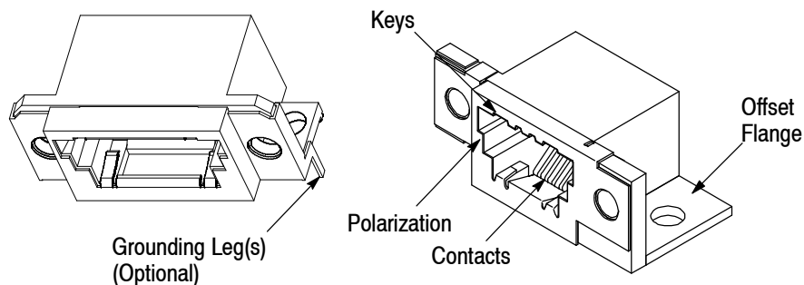
Side-Entry Receptacle (Typ)
