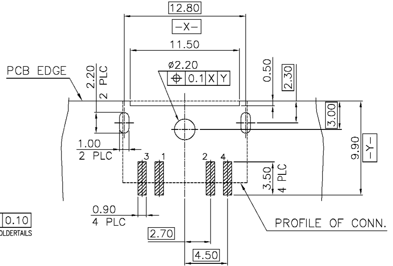
RECOMMENDED PCB LAYOUT (TOP VIEW) TOLERANCE: \pm 0.05 (THICKNESS=1.2mm)
