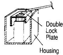
Detail C
