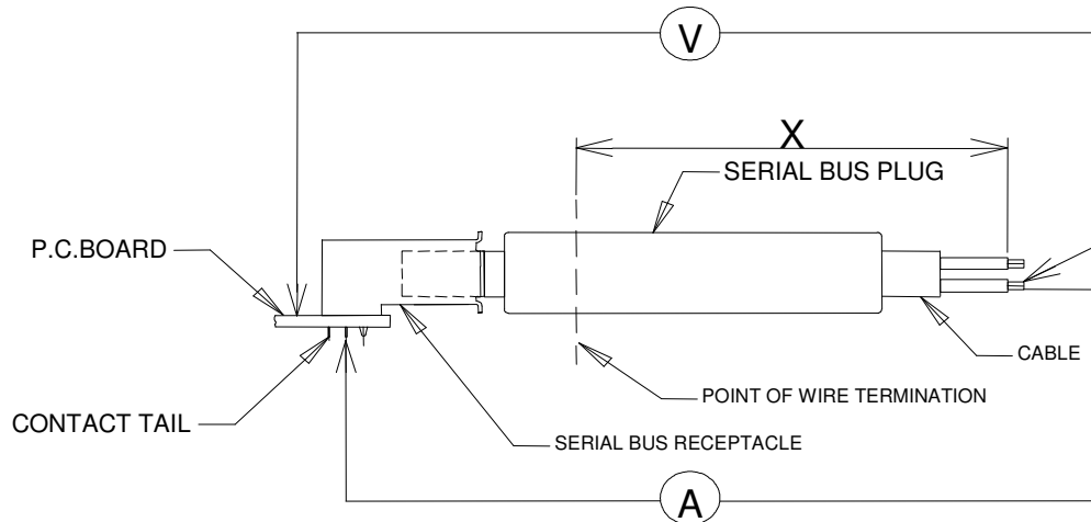
Figure 1 Typical Termination Resistance Measurement Points
