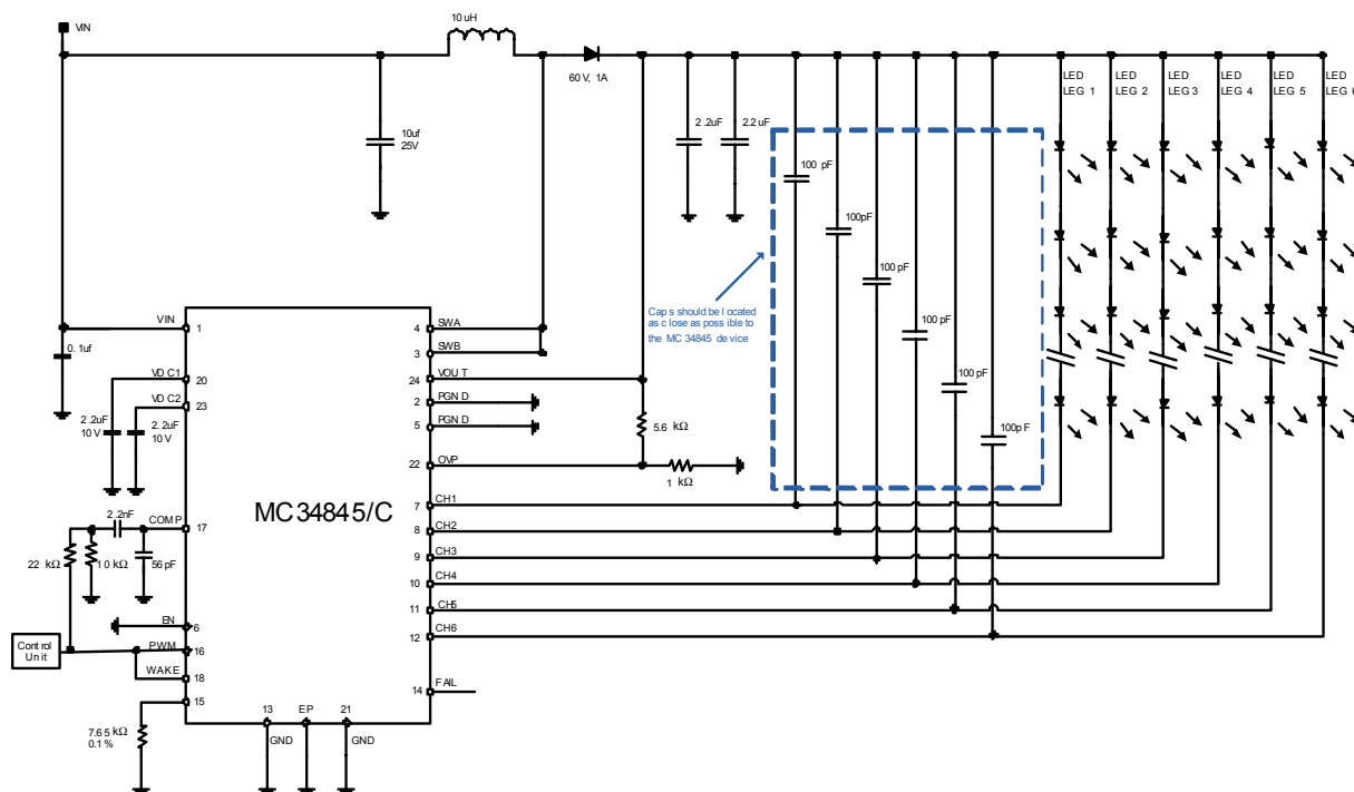
Figure 10. Typical Application Circuit for Single Wire Control, f_s = 600 \text{ KHz} ( V_{IN} = 9.0\text{V} , I_{LED}/\text{channel} = 20 \text{ mA/channel} , 12 LEDs/channel, OVP = 45\text{V} , V_{PWM} = 3.3\text{V} )
