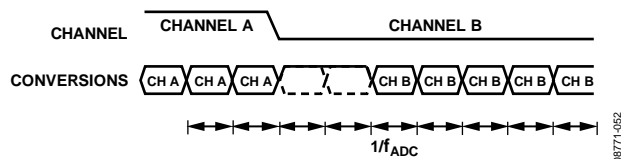
Figure 41. Channel Change ( \text{Sinc}^4 Chop Enabled)
