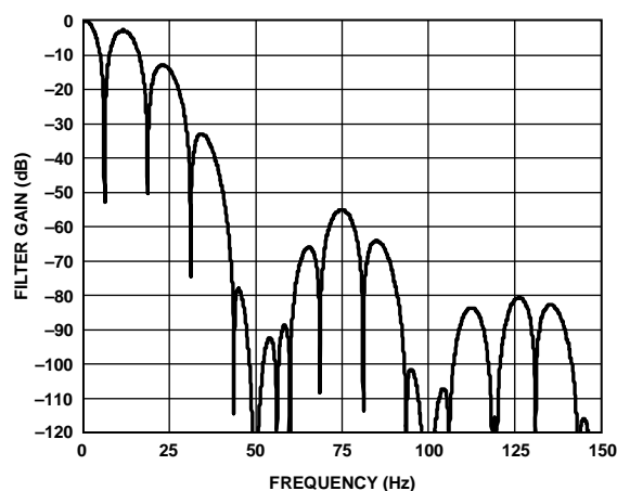
Figure 44. \text{Sinc}^4 Filter Response (FS[9:0] = 96, Chop Enabled, REJ60 = 1)
