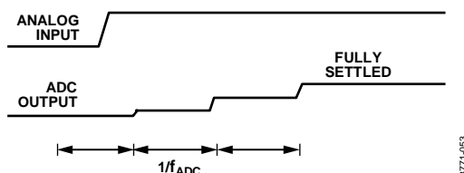
Figure 42. Asynchronous Step Change in Analog Input ( \text{Sinc}^4 Chop Enabled)
