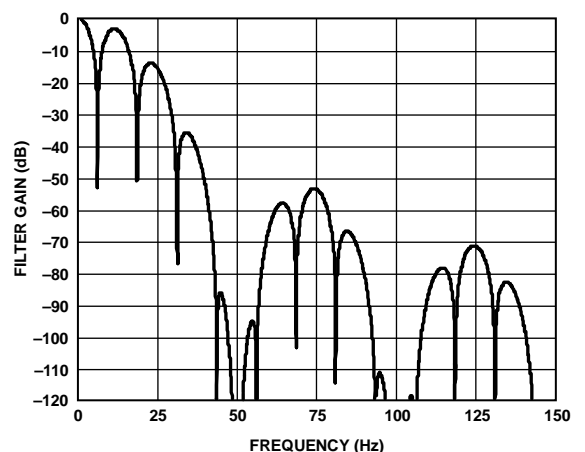
Figure 43. \text{Sinc}^4 Filter Response (FS[9:0] = 96, Chop Enabled)
