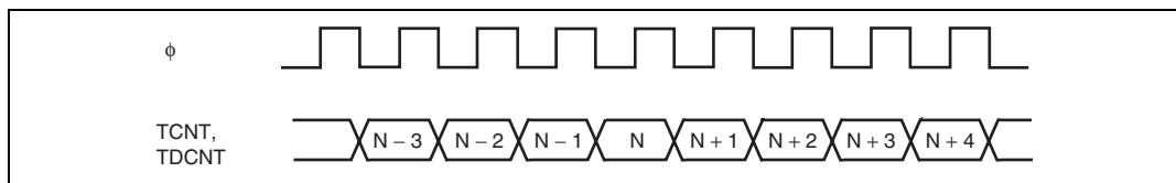
Figure 11.9 Count Timing
