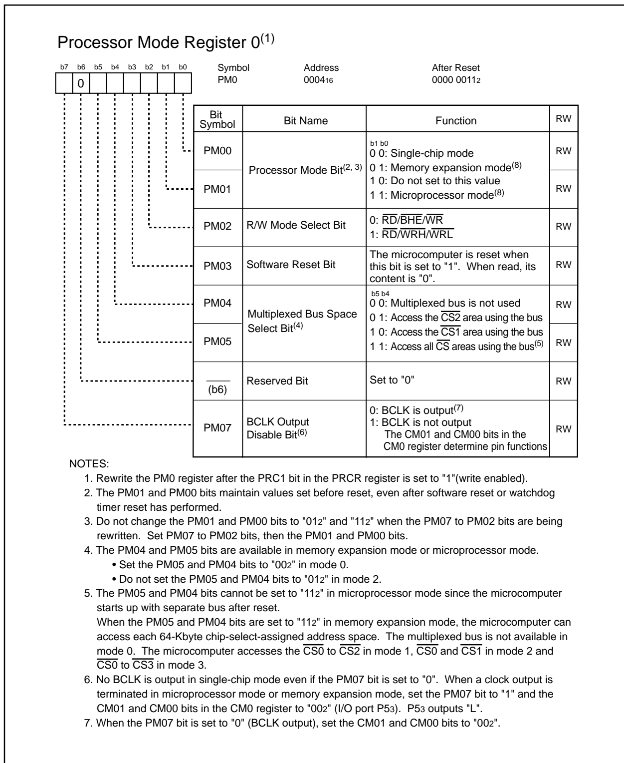
Figure 6.1 PM0 Register
