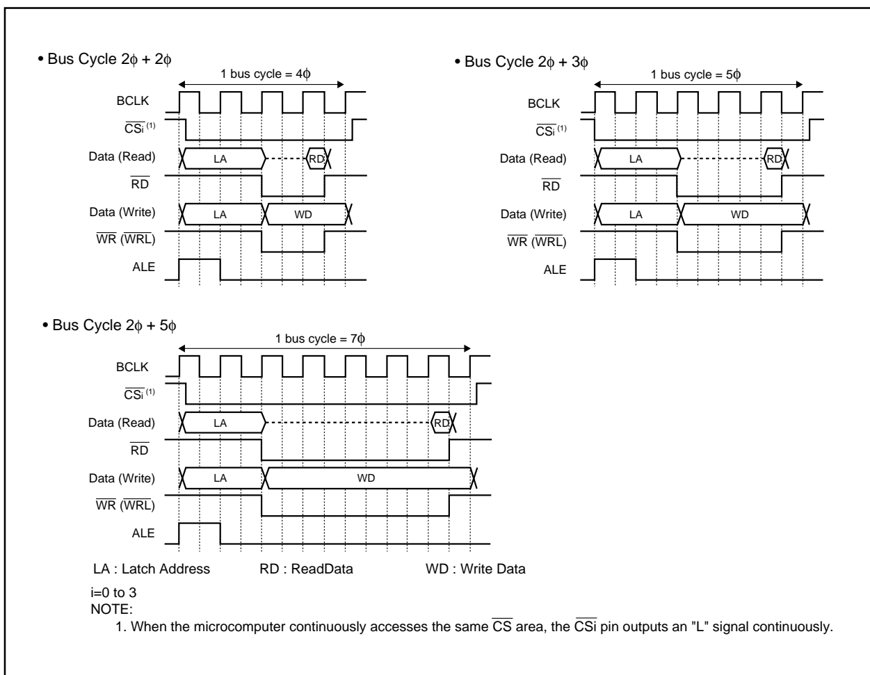
Figure 7.7 Bus Cycle with Multiplexed Bus (1)
