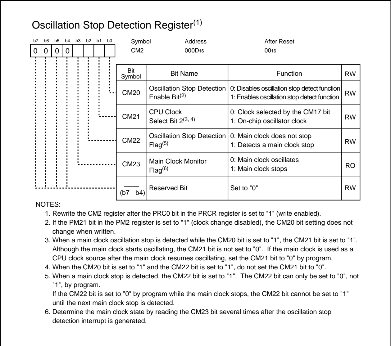
Figure 8.5 CM2 Register
